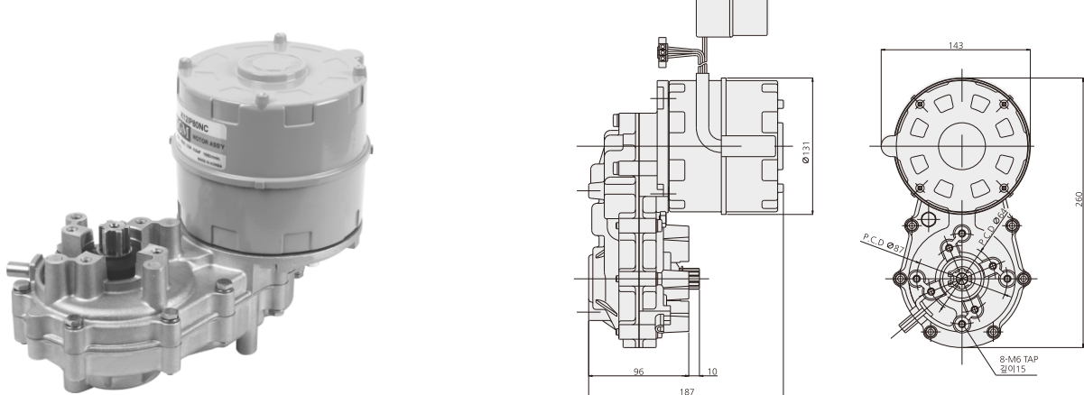
K12IP80N□ + KGJ SERIES
